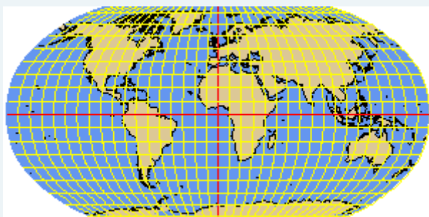
ROBINSON interpolated
