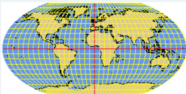
WAGNER6 elliptical
